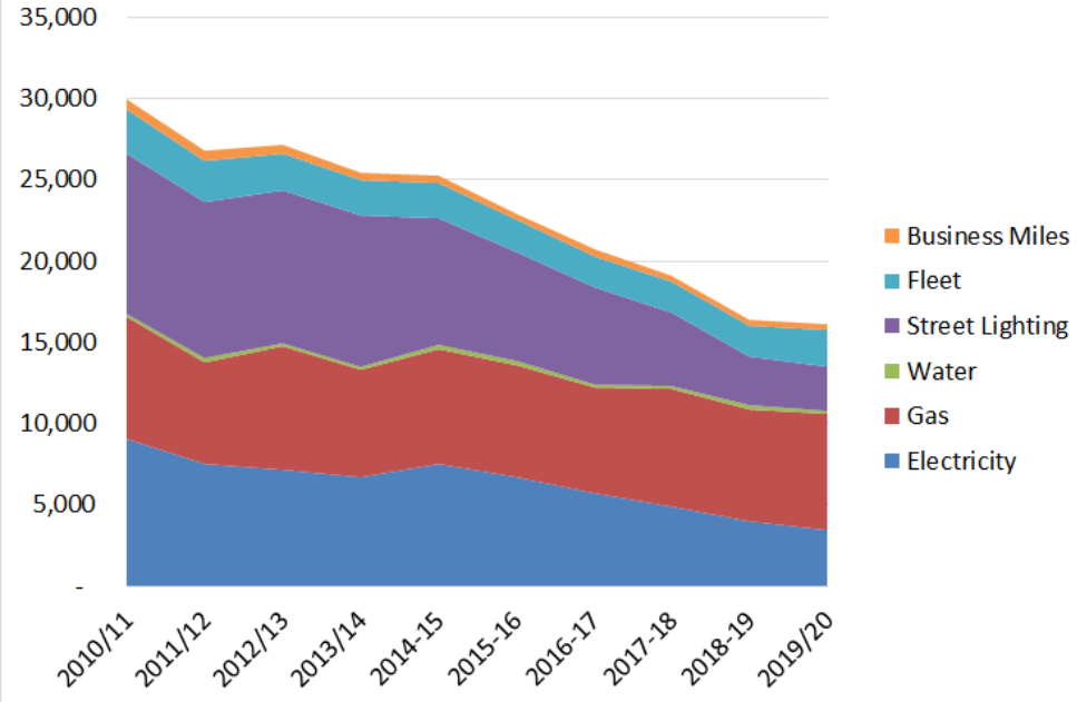
NTC CO 2 e emissions 2019-20 - 16,134 tonnes
