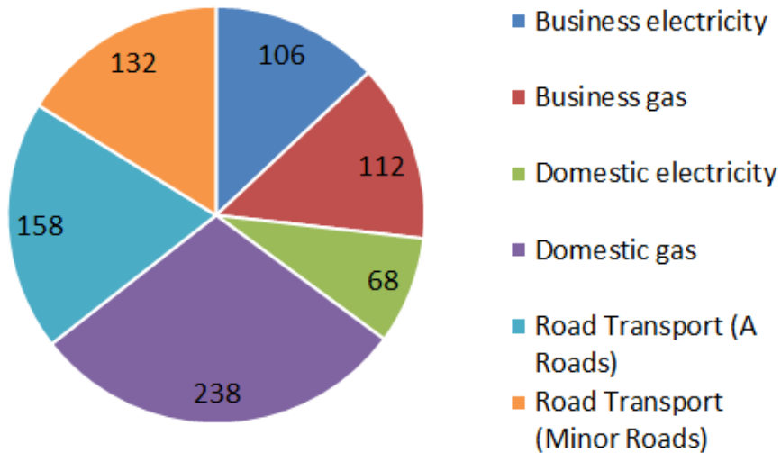
North Tyneside Borough carbon footprint 2018
