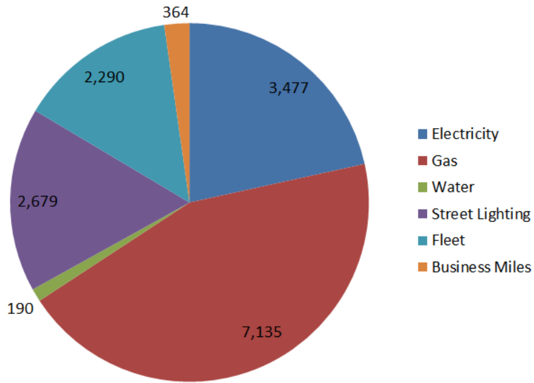
NTC CO 2 e emissions 2019-20 - 16,134 tonnes
