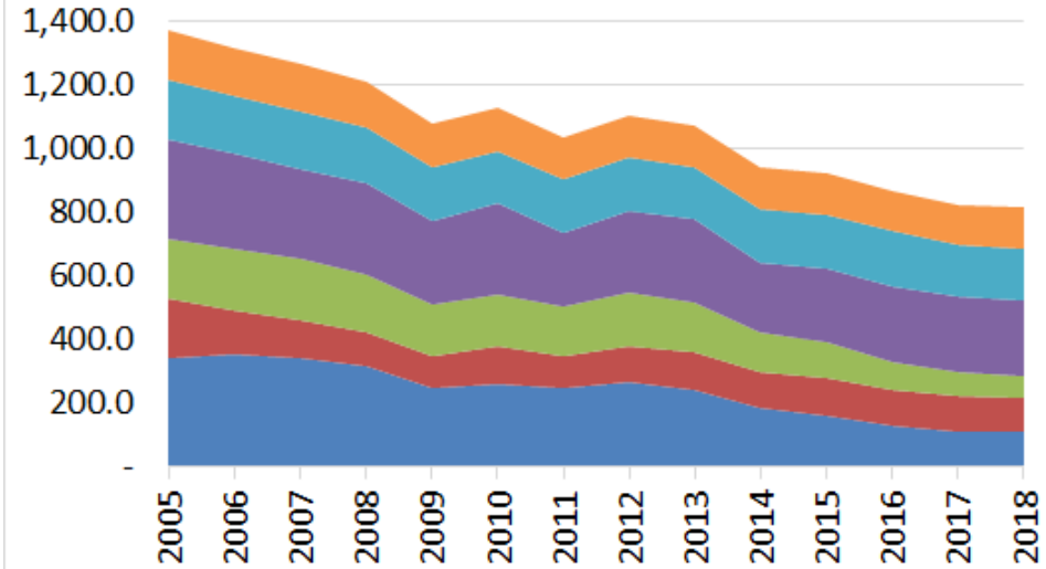
North Tyneside Borough carbon footprint 2005 - 2018
