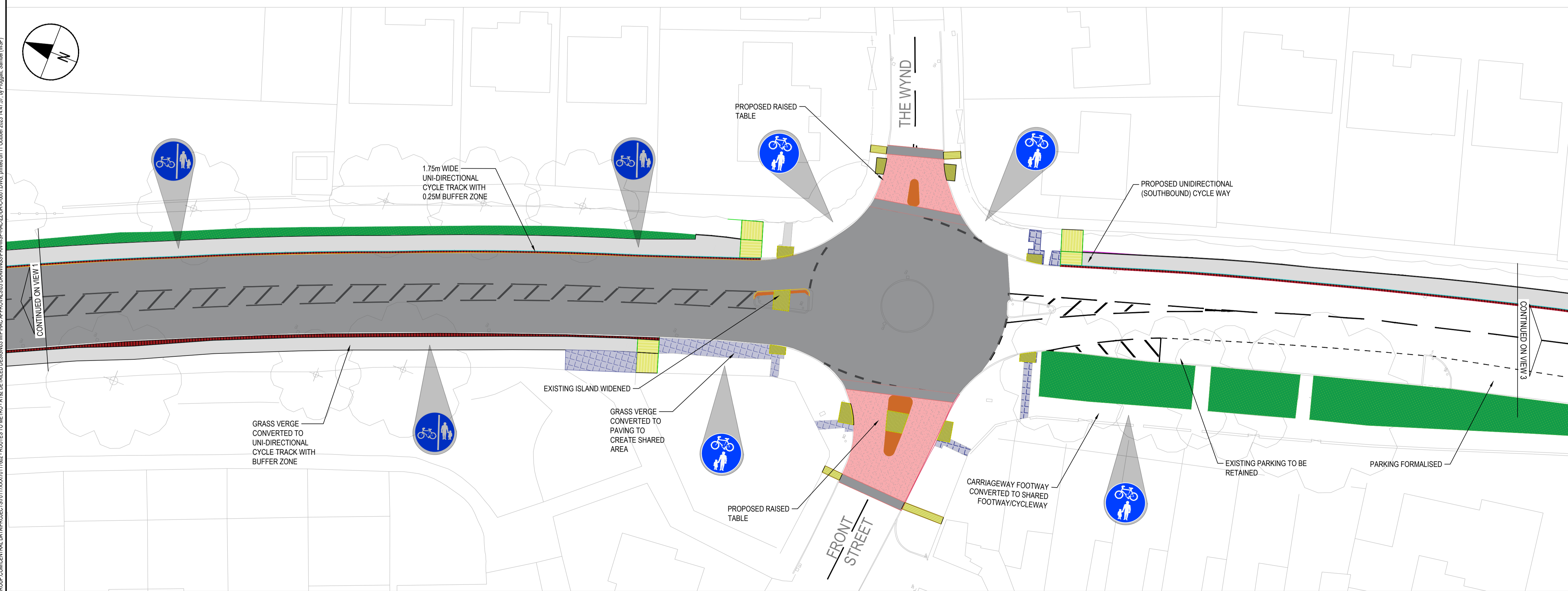
VIEW 2 SCALE 1:250
